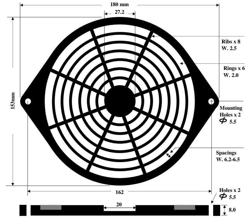
Guard "G" / G172P
